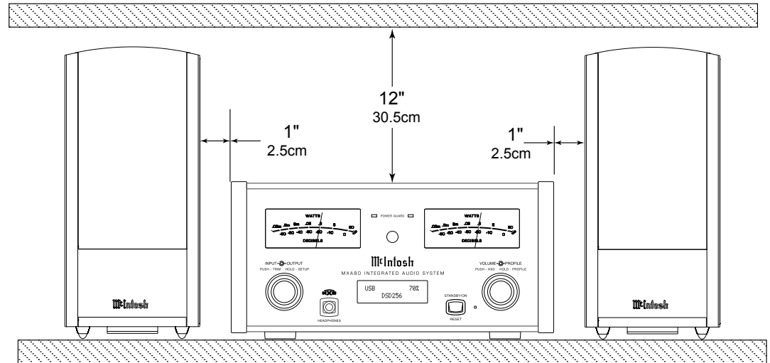
MXA80 Front View
