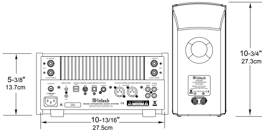
Rear View of the MXA80
