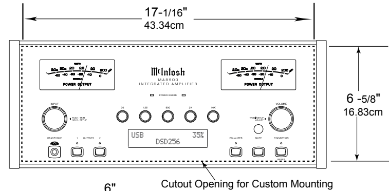
MA8900 Front Panel Custom Cabinet Cutout
