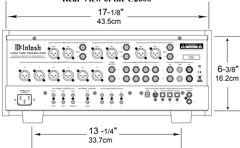
Rear View of the C2600
