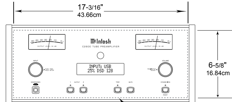
C2600 Front Panel Custom Cabinet Cutout
