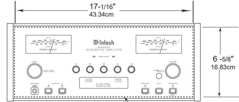
MA8950 Front Panel Custom Cabinet Cutout
