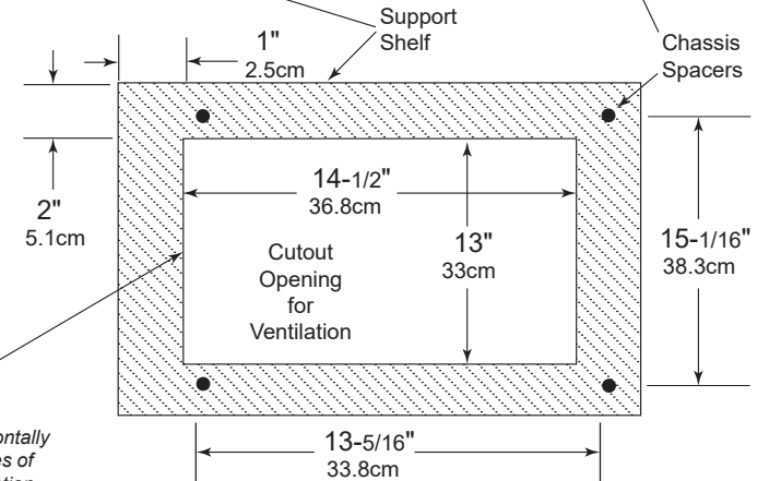
MA8950 Bottom View in Custom Cabinet
