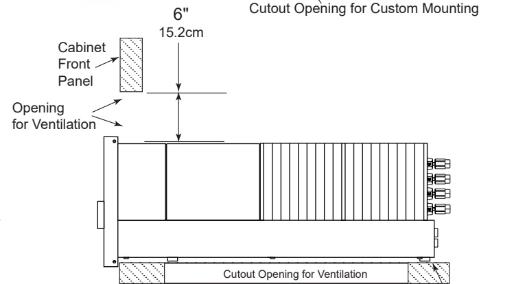
MA8950 Side View in Custom Cabinet
