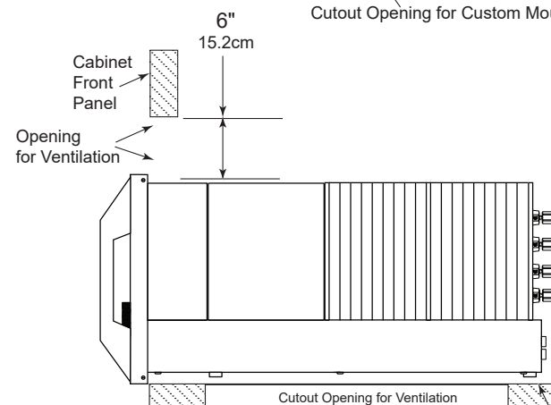
MA9500 Side View in Cabinet Cabinet
