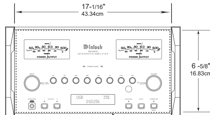
MA9500 Front Panel Custom Cabinet Cutout
