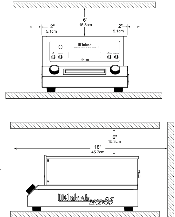
Figure 02– Ventilation requirements
