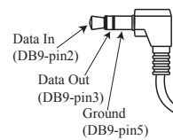
Figure 06– Mini plug for RS232 connection
