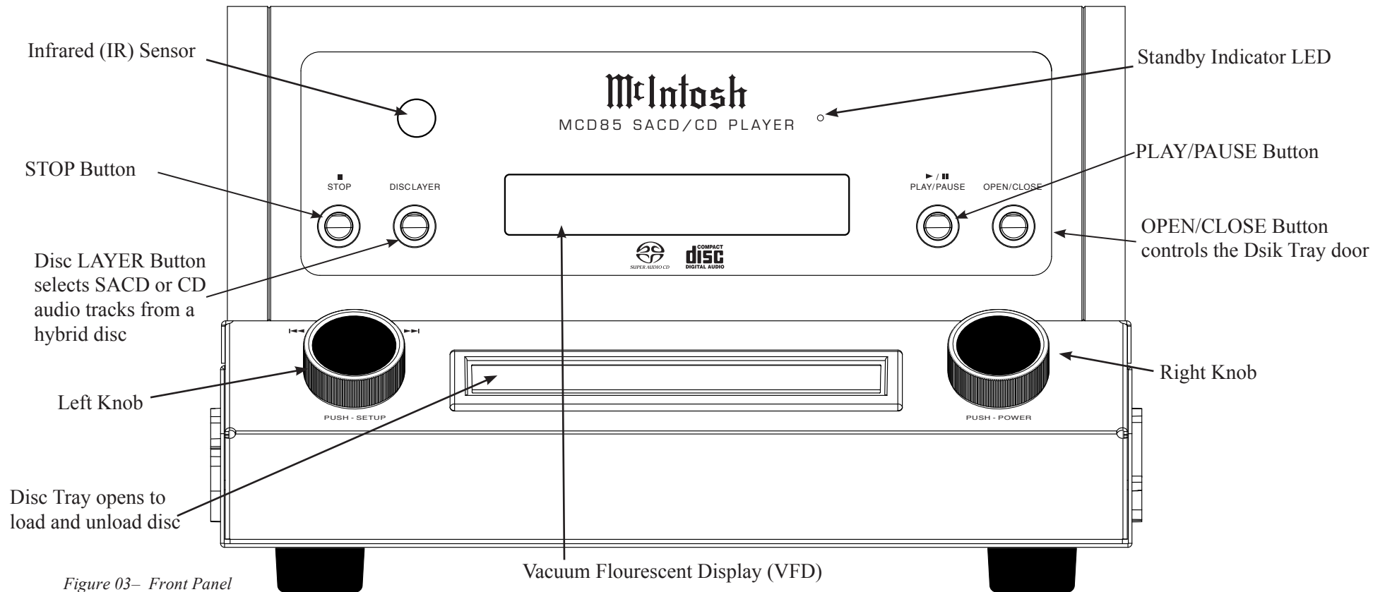
Figure 03– Front Panel
