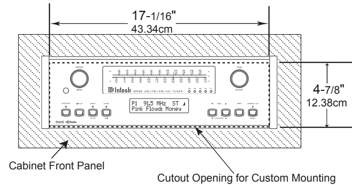
MR88 Front Panel Custom Cabinet Cutout
