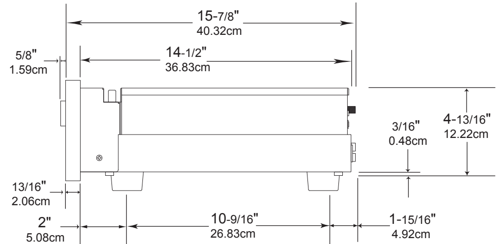
Side View of the MR88
