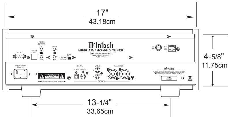
Rear View of the MR88
