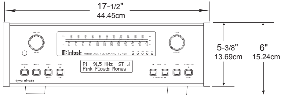
Front View of the MR88
